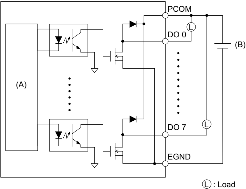
(A) Circuit interne (B) 24 Vcc
