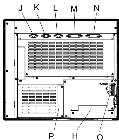
PL-7900T(4Slot)
