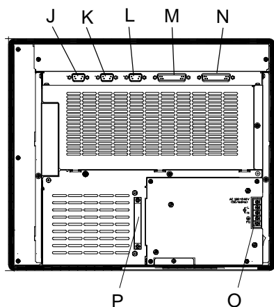
PL-7901T(2Slot)
