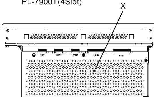
PL-7900T(4Slot)
