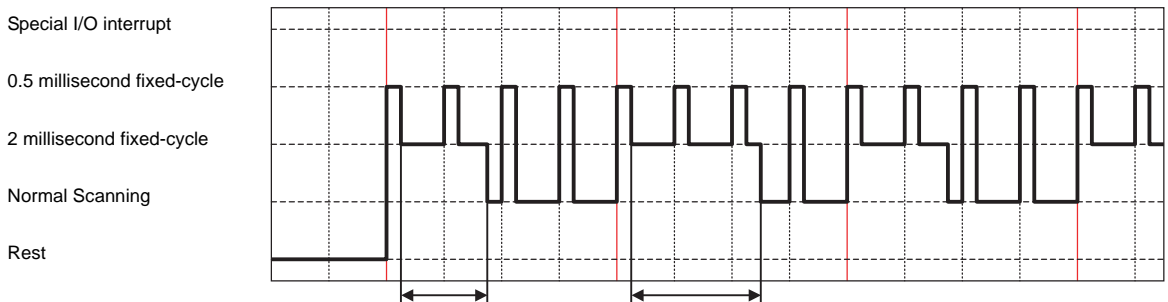
Depending on the special I/O processing, the processing time of the fixed-cycle varies. The normal scanning time is affected.
