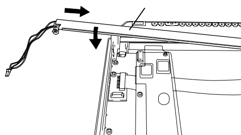
Backlight Unit
