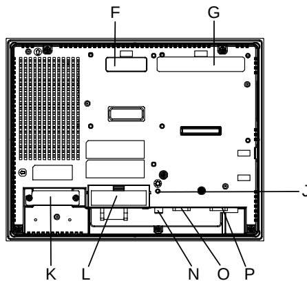
Back (AGP-35*0T)
