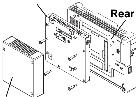
Expansion Unit
