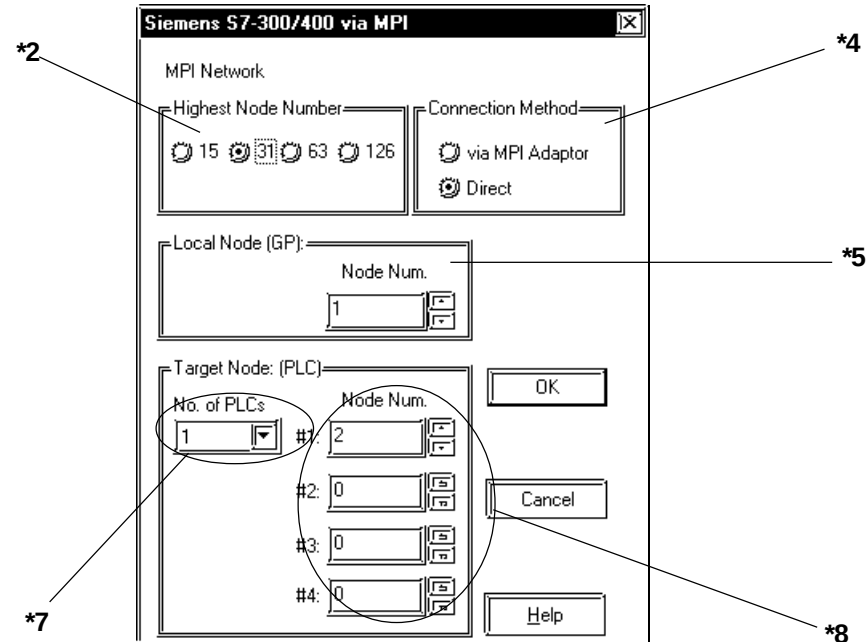
<SIMATIC S7-300/400 Series MPI Network Setting Window>
