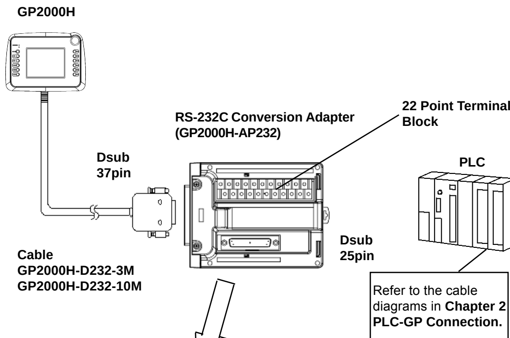
Dsub Connector
