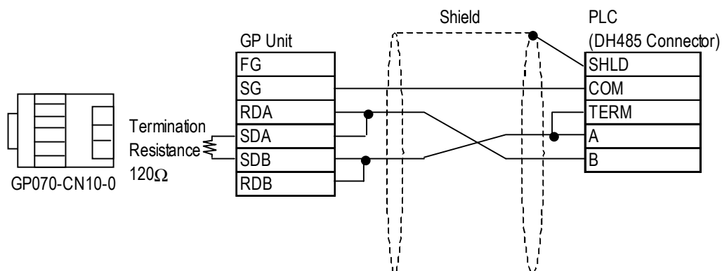
Cable Diagram 4 (RS-422C)
