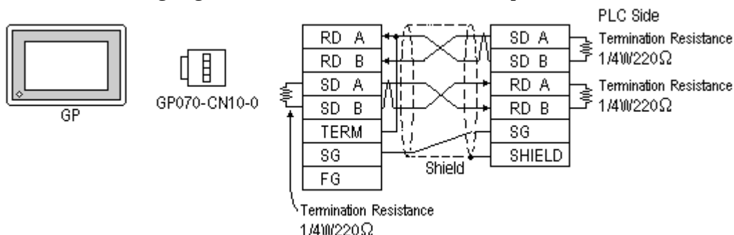
Cable Diagram 2 (RS-422)
