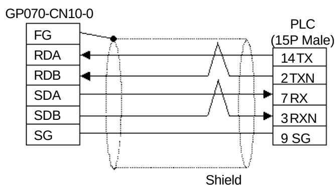
Cable Diagram 7 (RS-422, 4-wire)
