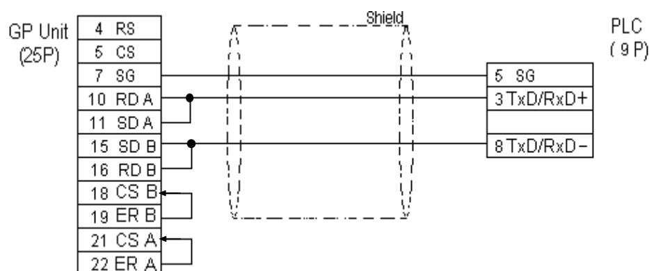
Cable Diagram 2 (RS-422)
