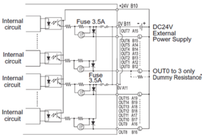
Output Circuit Sink Type
