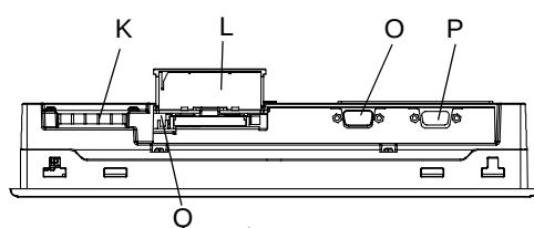
底面図 (AGP-3500L/3500S)
