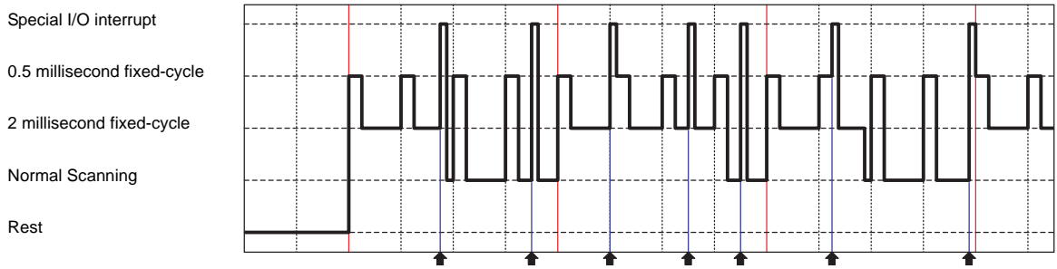
The special I/O processing affects the processing time of 0.5 milliseconds fixed-cycle and the normal scanning time.
